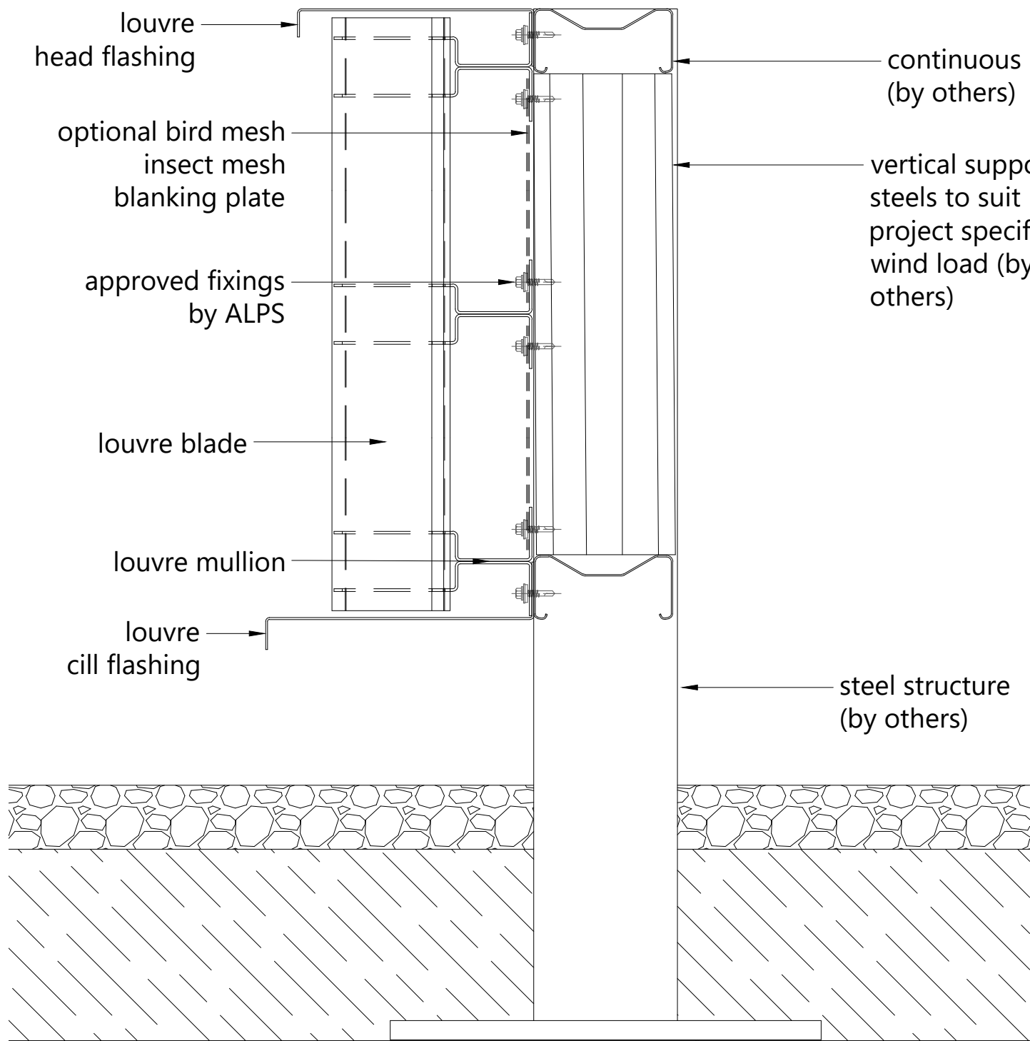
Typical 1UL/MV Section
