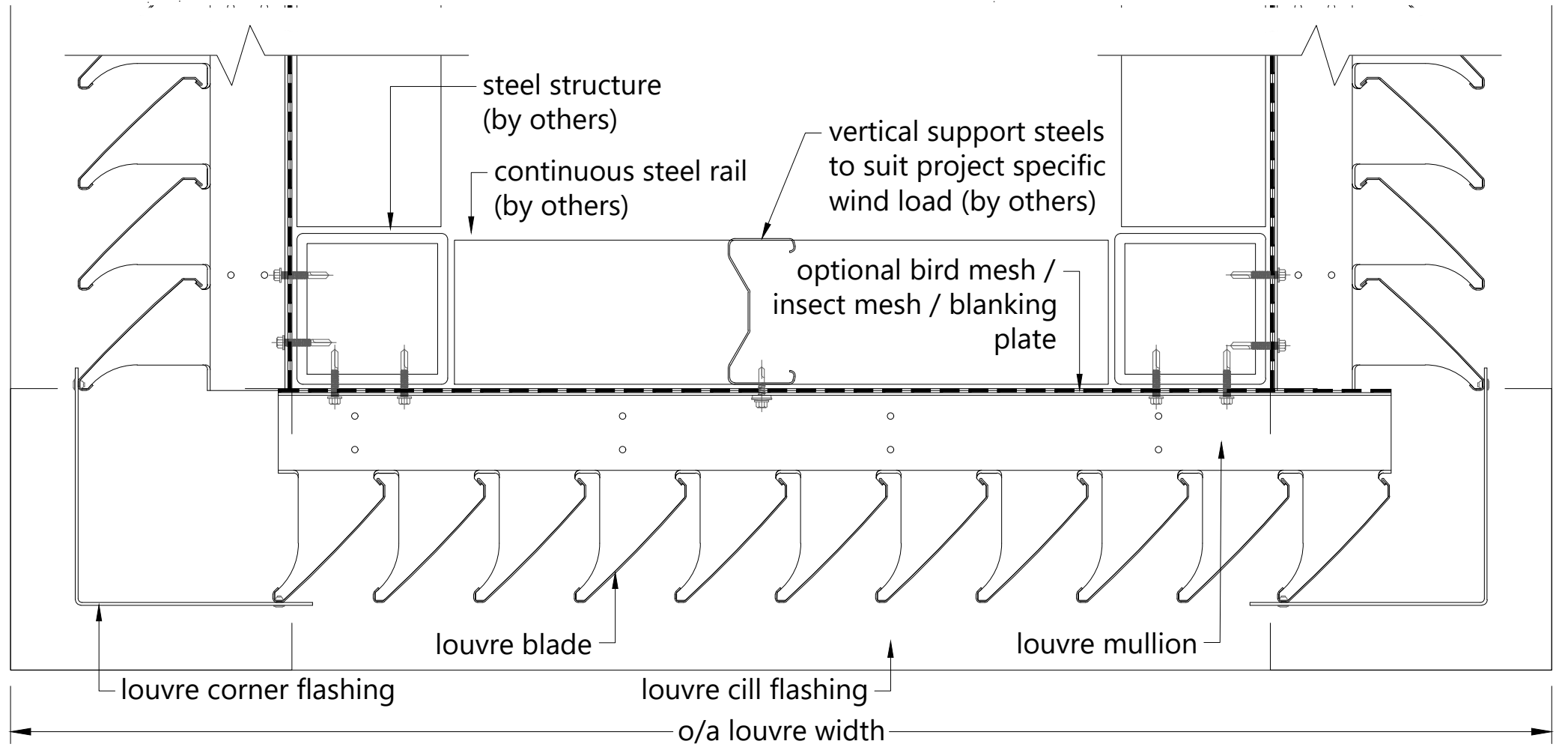
Typical 1UL/MV Plan
