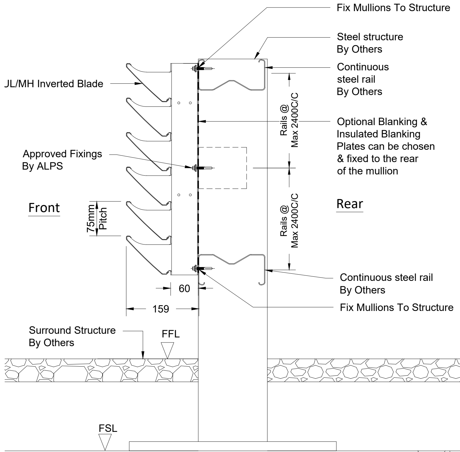
Typical 1ULMH Inverted Section
