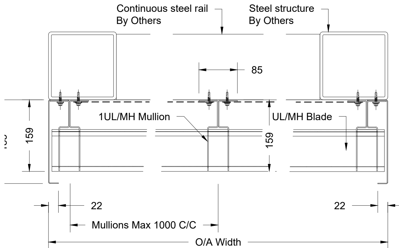
Typical 1ULMH Inverted Plan
