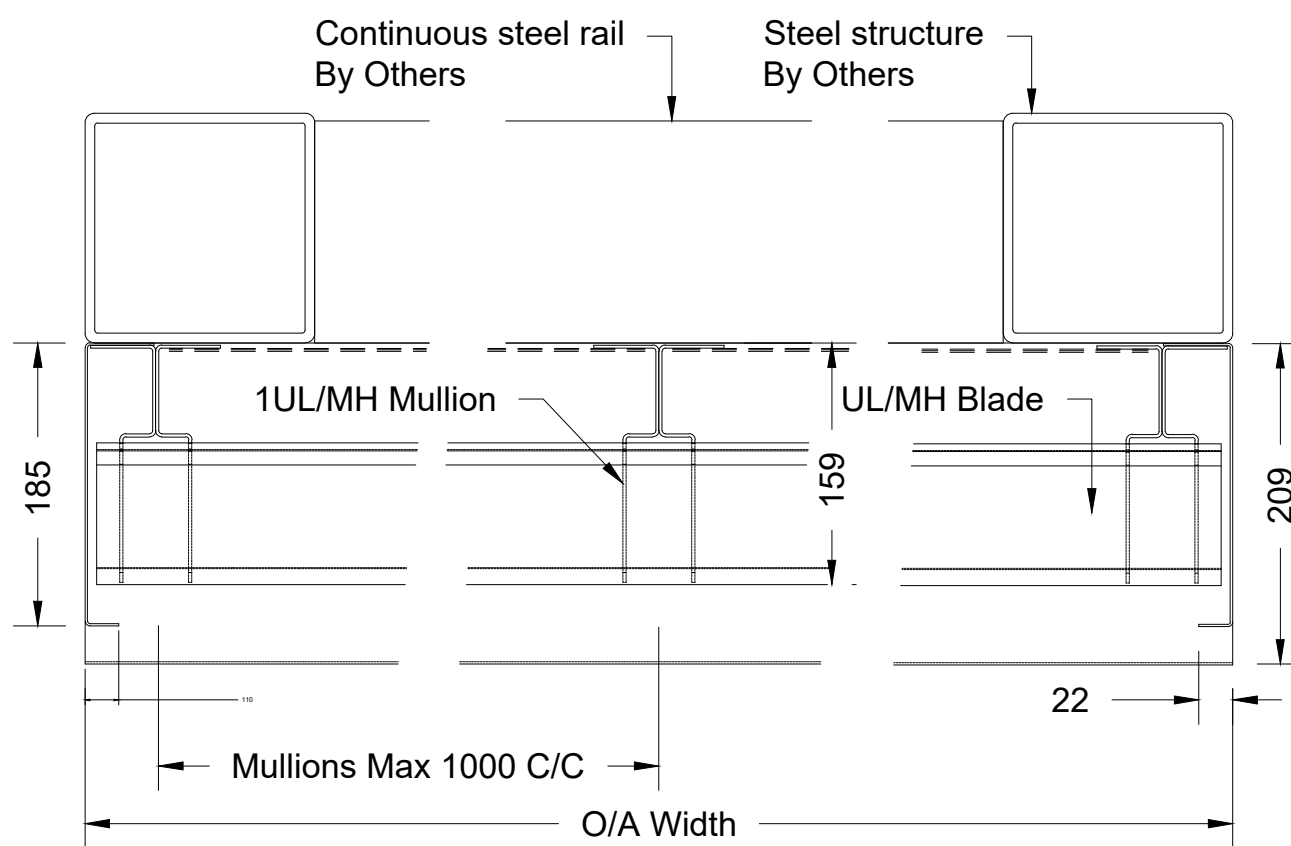
Typical 1ULMH Plan
