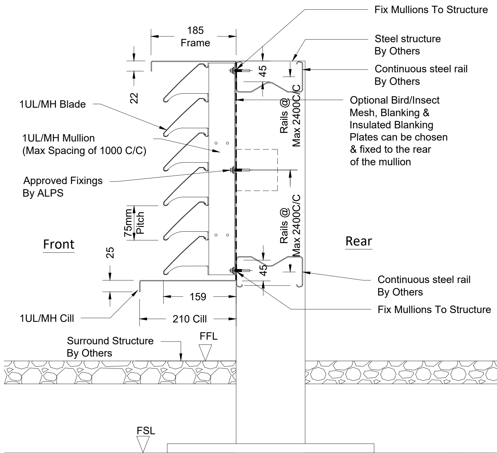
Typical 1ULMH Section
